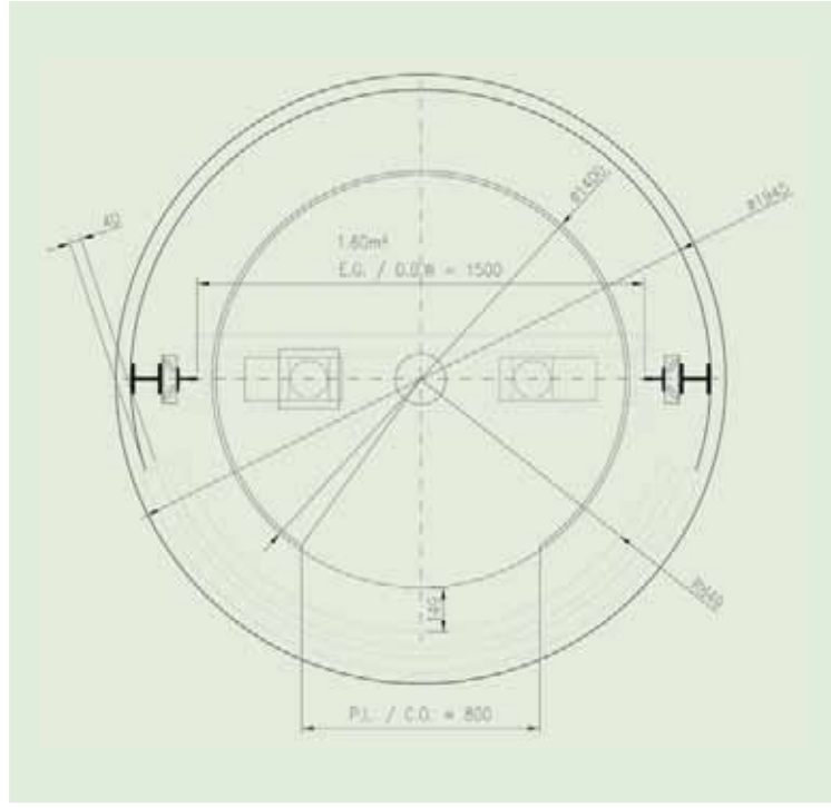
Ascensor circular. Circular lift.
