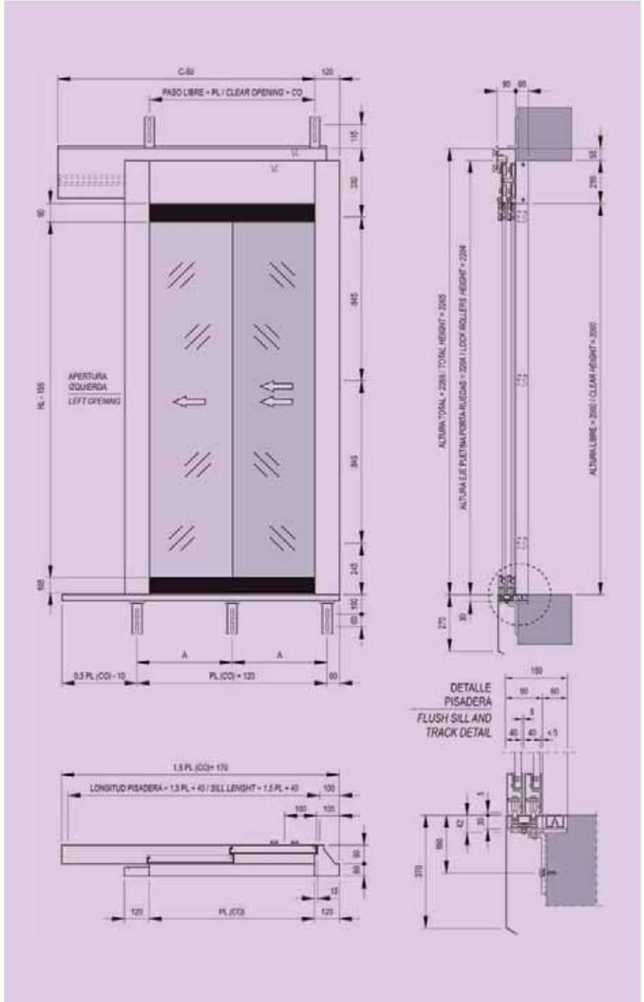
Puerta cristal total. Complete glass door.
