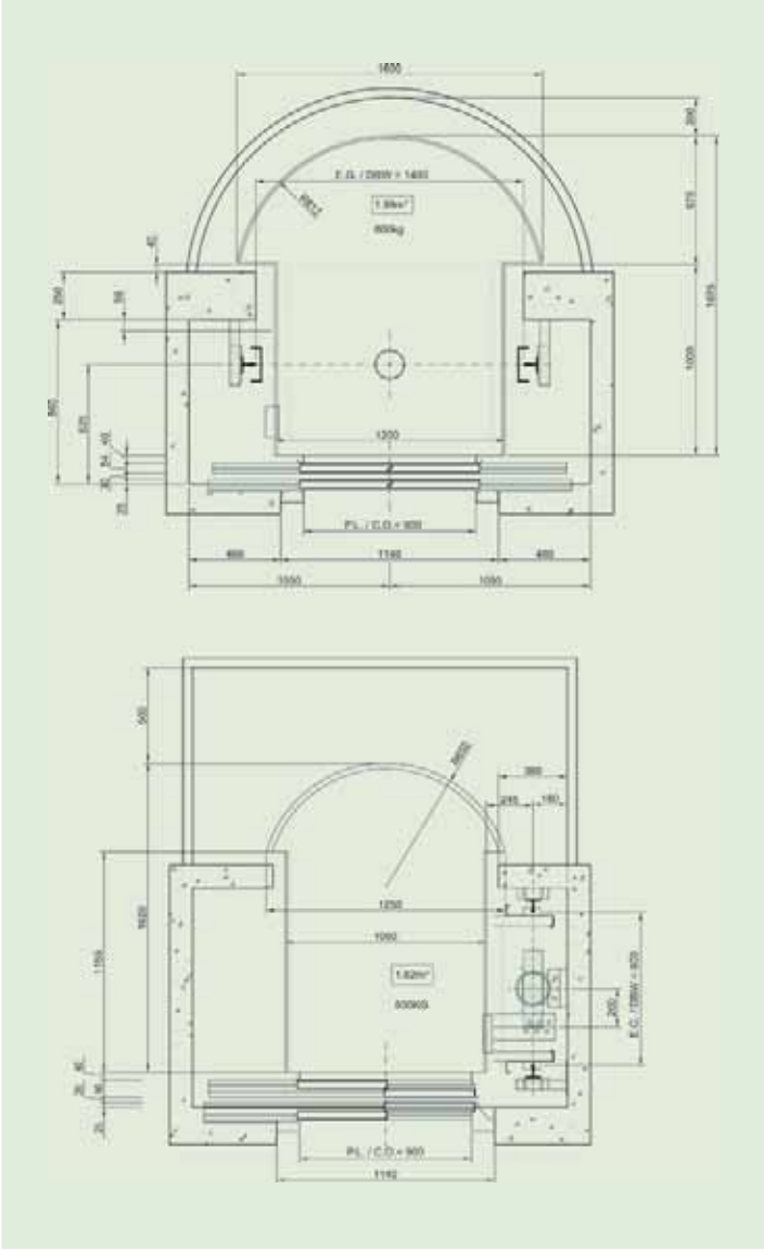
Ascensor con cabina semicircular adaptada a hueco. Lift with semicircular car adapted to shaft.
