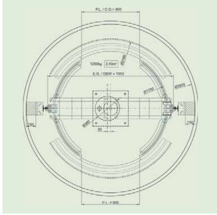
Ascensor circular. Circular lift.
